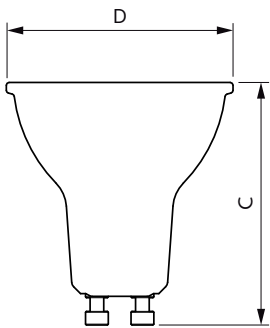
GU10 220-240V 6.7-90W 670lm 60D 3000KND
