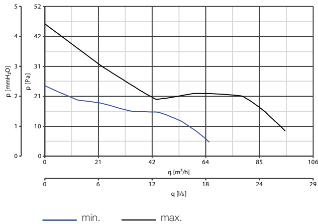
ME 100/4" LL
