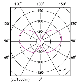
Light Distribution Diagram - MAS LEDBulbND4-60W E27 827 G95 CL G UE
